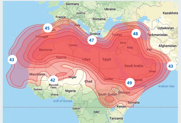
Footprint (G/T) dB/K
