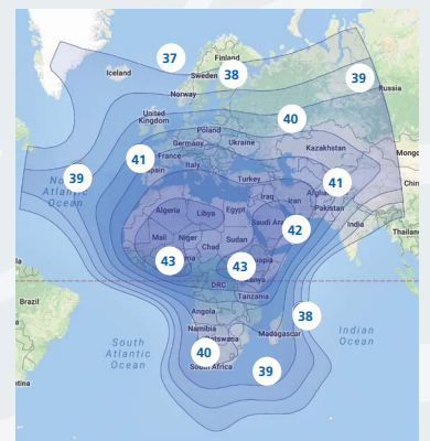
Footprint (G/T) dB/K
