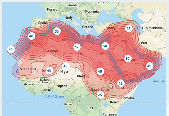
Footprint (G/T) dB/K
