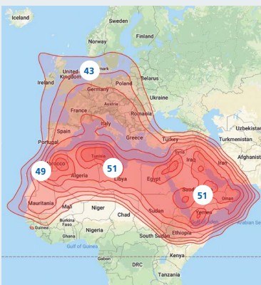
Footprint (G/T) dB/K
