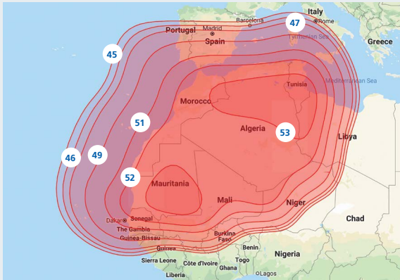
Footprint (G/T) dB/K
